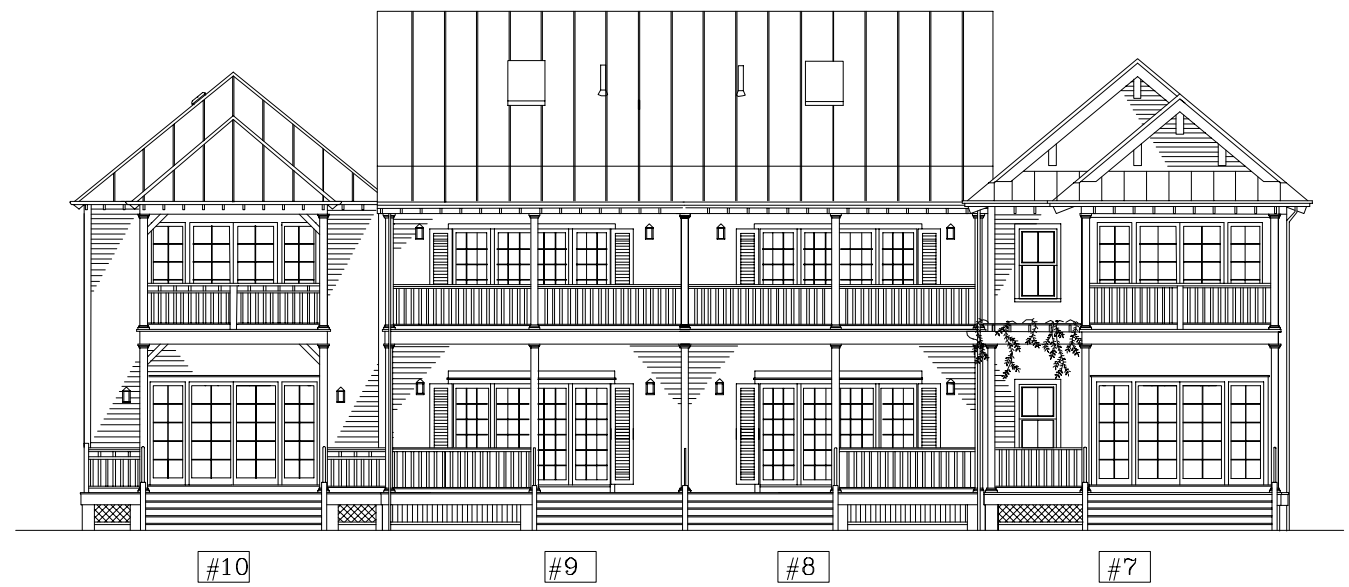
UNITS 7-10 REAR ELEVATIONS
