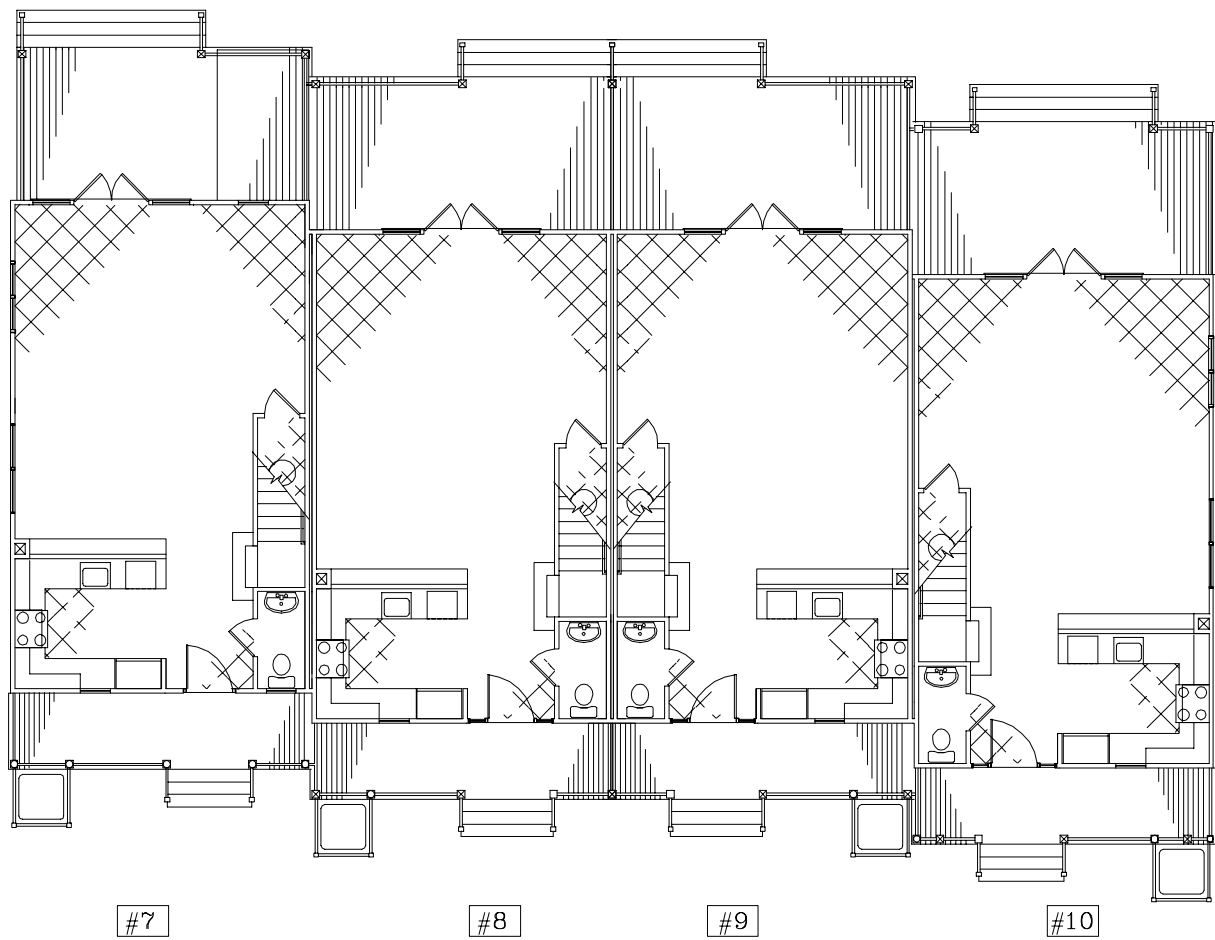
UNITS 7-10 FIRST FLOOR PLANS
