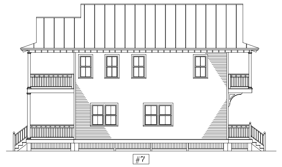
UNIT 7 SIDE ELEVATION
