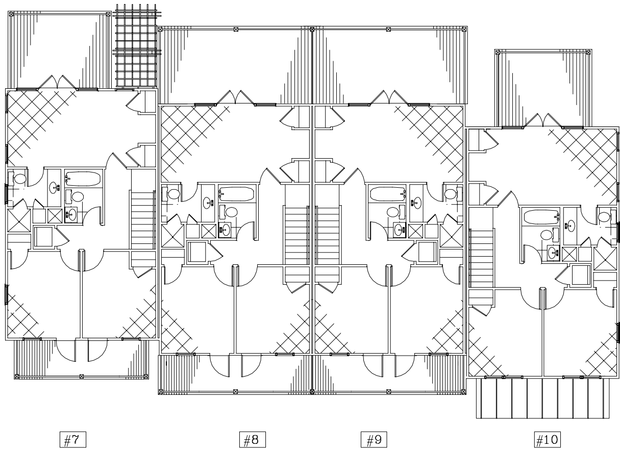
UNITS 7-10 SECOND FLOOR PLANS
