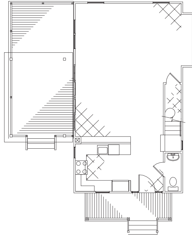
UNIT 25 - FIRST FLOOR PLAN
