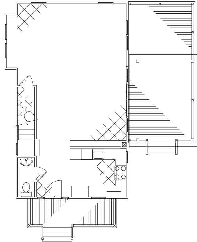
UNIT 24 - FIRST FLOOR PLAN
