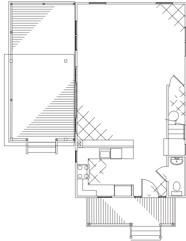
UNIT 23 - FIRST FLOOR PLAN
