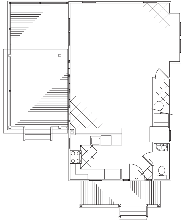
UNIT 21 - FIRST FLOOR PLAN
