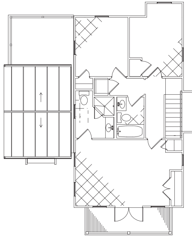
UNIT 19 - SECOND FLOOR PLAN
