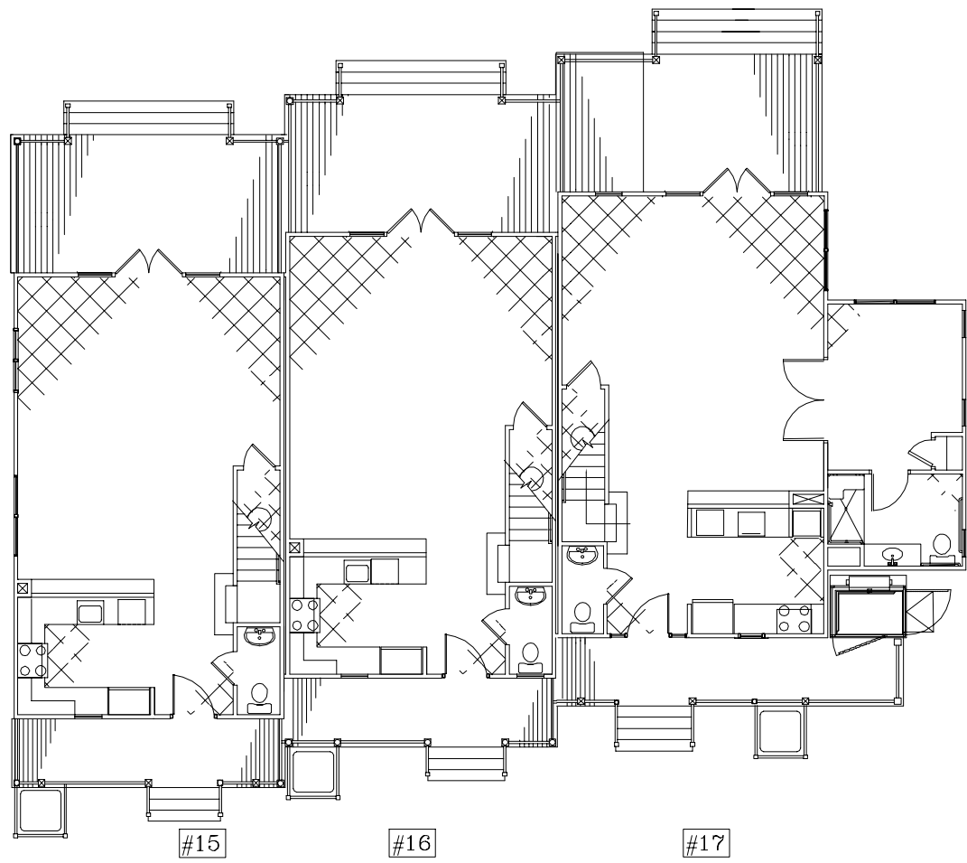
UNITS 15-17 FIRST FLOOR PLANS
