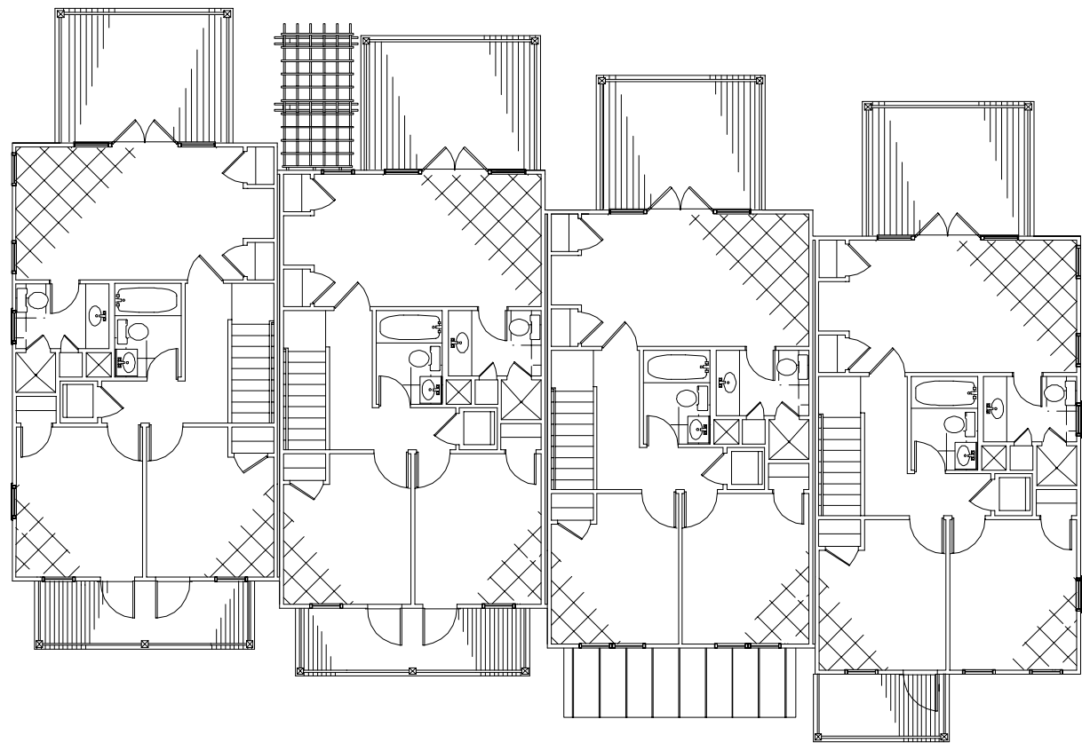
UNITS 11-14 SECOND FLOOR PLANS
